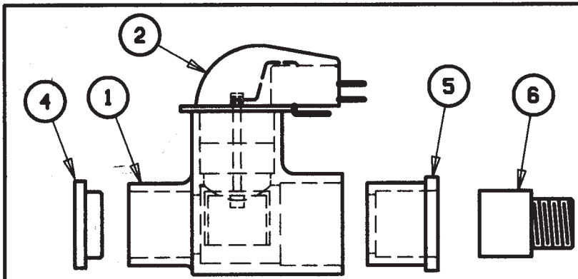
HORIZONTAL APPLICATION
