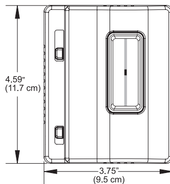
Vertical design
