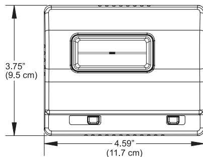
Horizontal design
