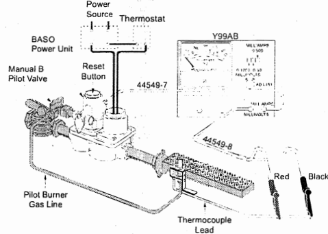
Figure 2: Turn Down Test Using Y99AB Test Kit
