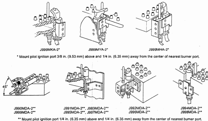
Figure 1: Possible Mounting Positions
